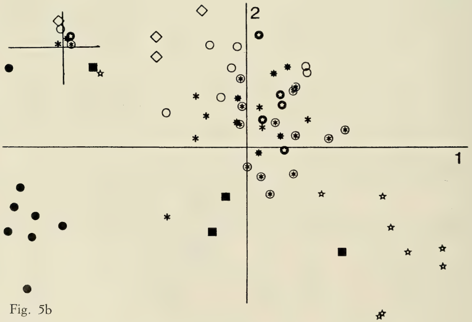
Fig. 5. Canonical variates plots showing relationships between Philoaterus from different localities. Individuals are plotted on the large axes and the means for each locality are shown on the smaller axes. a. Females; b. Males.
